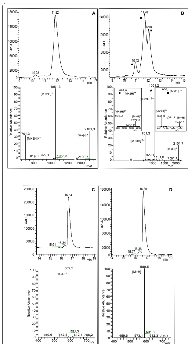
Figure 1 Reversed-phase high performance liquid chromatography (RP-HPLC) chromatograms and mass spectra at t = 0 and t = 24 h for RGDechiHCit (A and B) and c(RGDf[NMe]V) (C and D), respectively. In panel B the chromatographic peaks at t_r = 11.70 (Black Star), 12.04 (Black Square) and 10.93 min (Black Circle) are marked.
